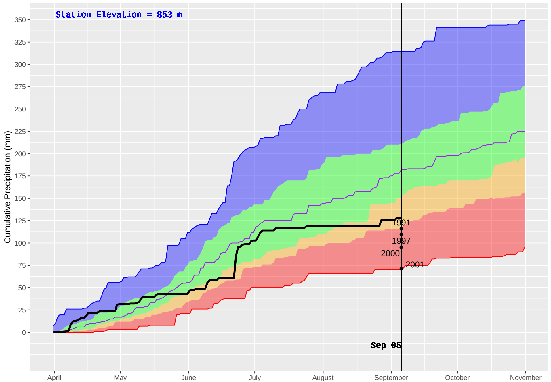
JOHNSON LAKE (419) : Historical (1986–2016) and Current (2018) Daily Cumulative Precipitation
