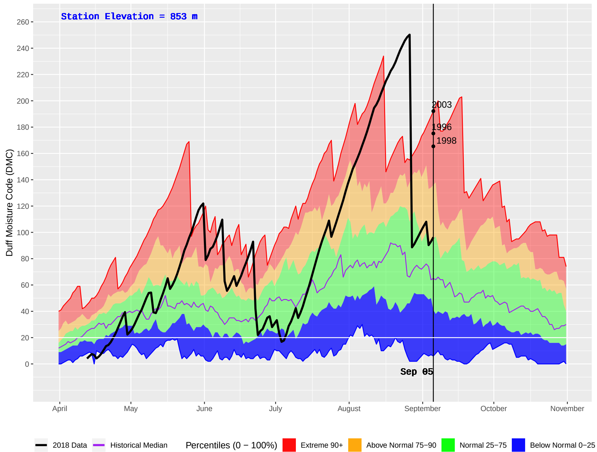
JOHNSON LAKE (419) : Historical (1986–2016) and Current (2018) Daily Duff Moisture Code (DMC)
