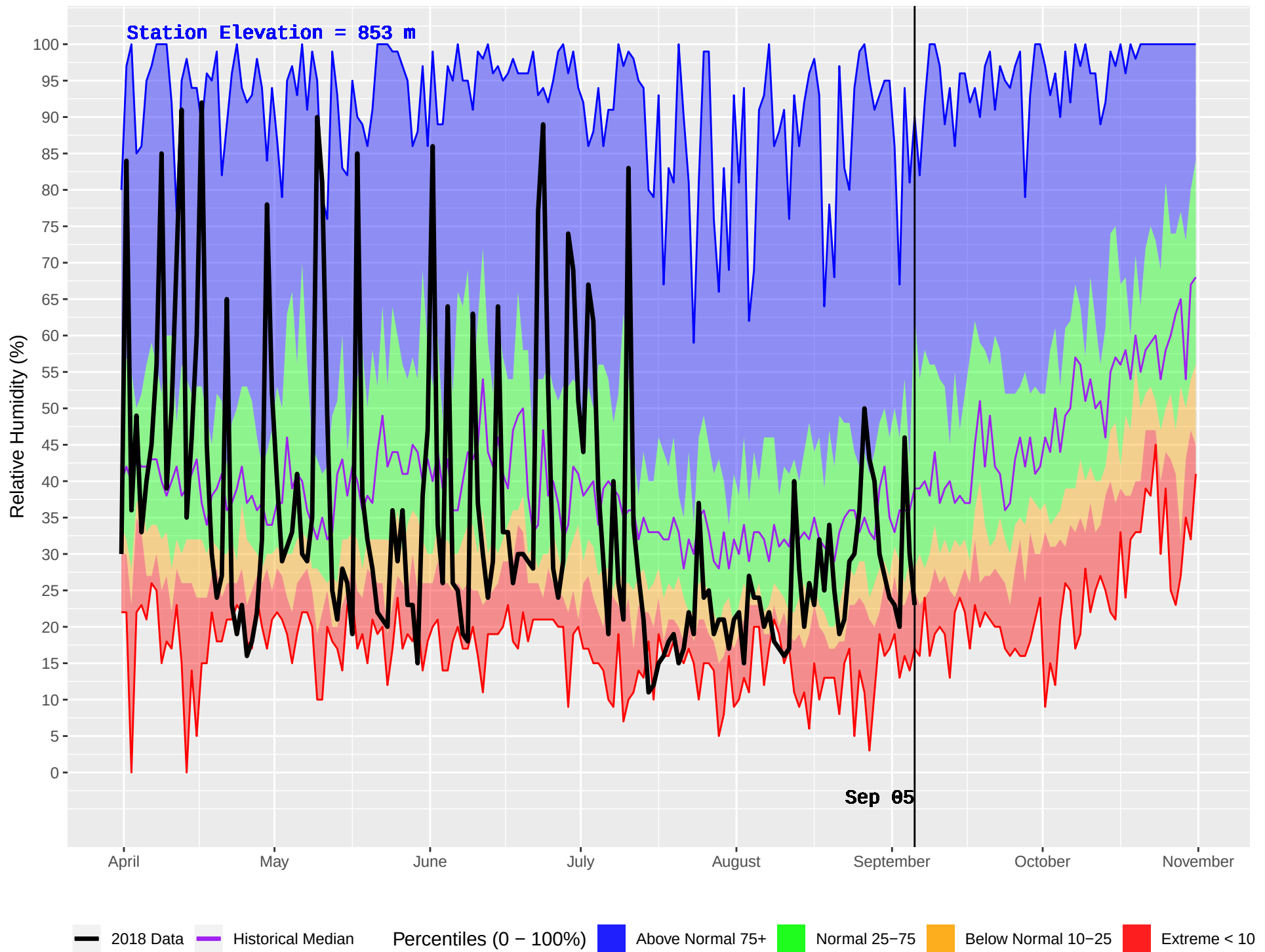
JOHNSON LAKE (419) : Historical (1986–2016) and Current (2018) Daily Relative Humidity
