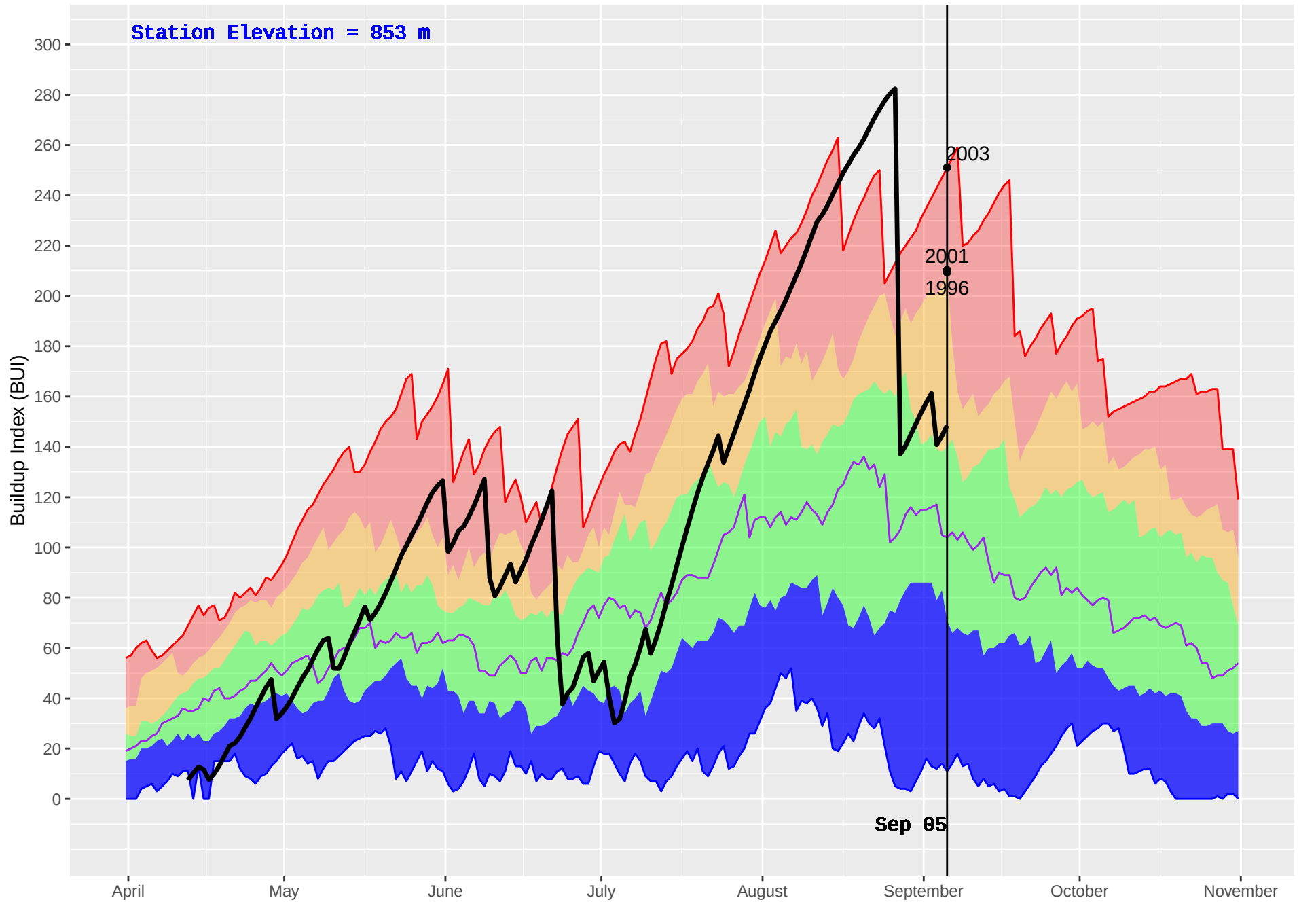
JOHNSON LAKE (419) : Historical (1986–2016) and Current (2018) Daily Buildup Index (BUI)
