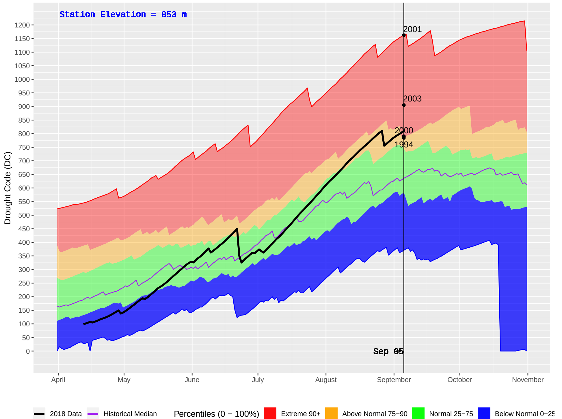
JOHNSON LAKE (419) : Historical (1986–2016) and Current (2018) Daily Drought Code (DC)
